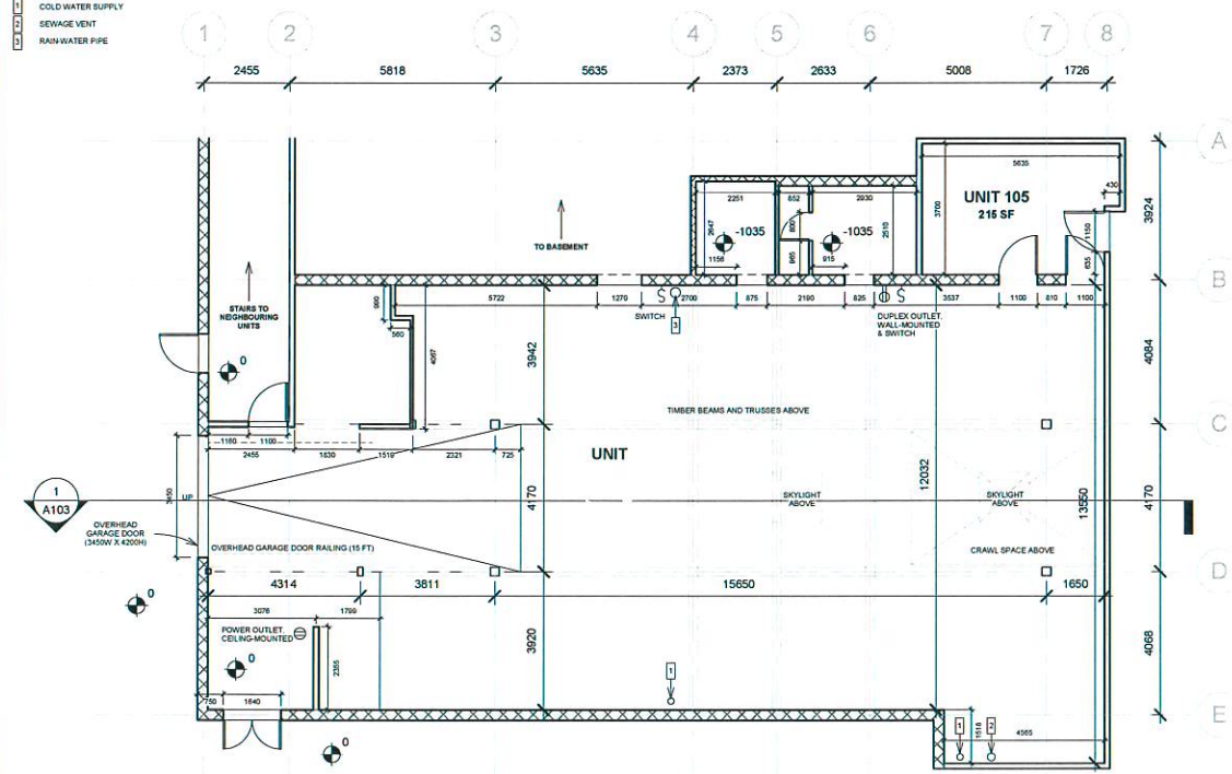
① Main Floor 1 : 100
